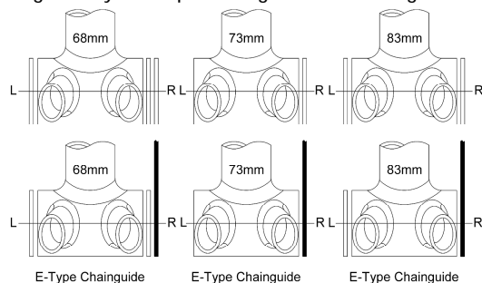
Fig.2: Alloy Shell Spacer Diagram for MTB MegaExo
